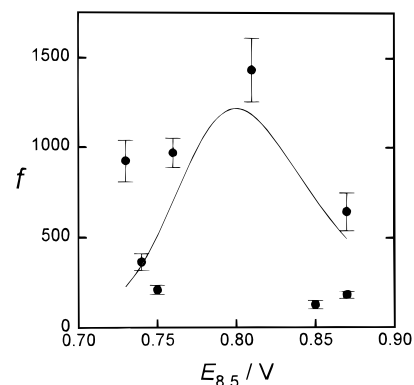
Figure 4. Relative enhancement efficiency of the phenolic compounds ( f ) as a function of the reduction potentials of the respective phenoxy radicals. The solid line is the curve calculated according to the model discussed in the text.
